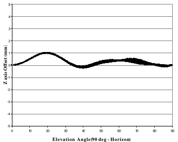
Figure 4. L1-L2 channel phase center offset variation in vertical plane for 12-arm L1/L2 antenna
