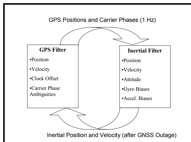
Figure 1. SPAN Tightly Coupled Architecture
