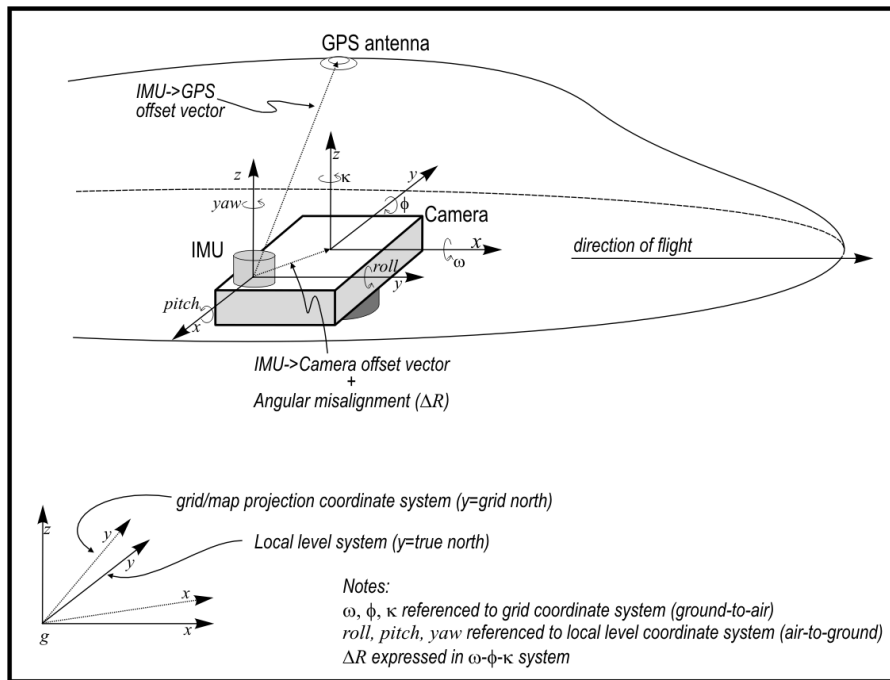
Figure 9. Relation of Omega-Phi-Kappa (WPK) to Roll-Pitch-Heading (RPH)
