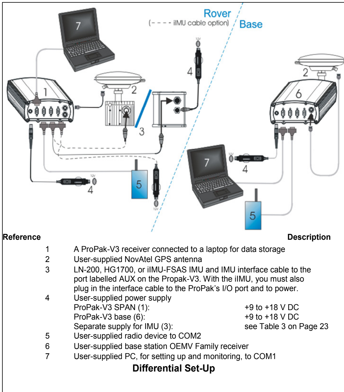
Figure 3. SPAN Setup with Differential Corrections
