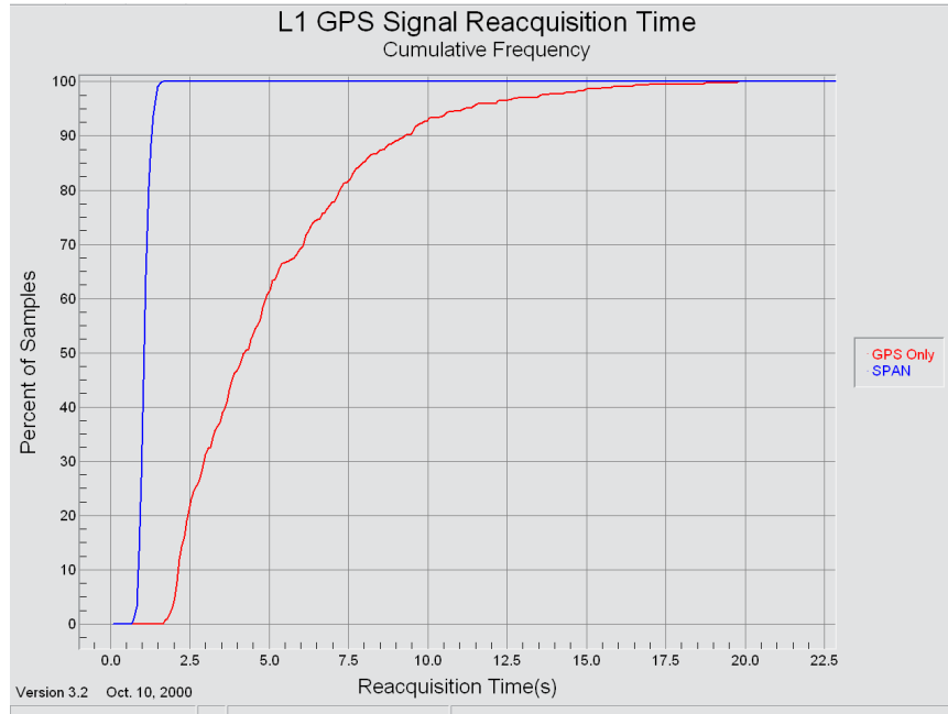
Figure 2. L1 GPS Signal Reacquisition with and without SPAN
