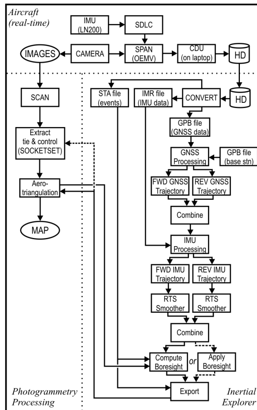
Figure 7. Workflow for Aerial Photo Mission Using Inertial Explorer and SPAN
