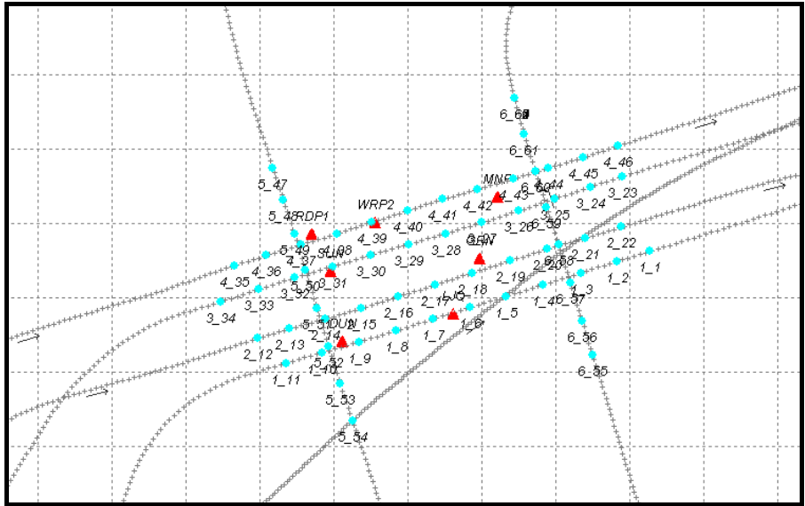
Figure 6. Flight Lines, Photo Points (cyan dots) and Ground Control Points (red triangles)
