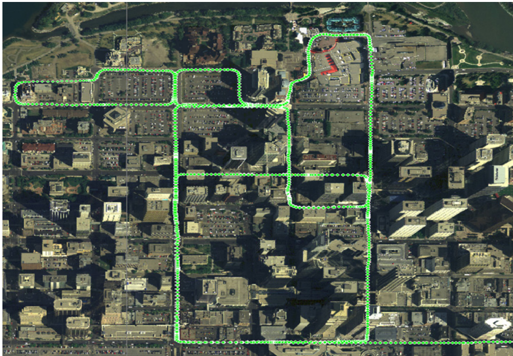
Figure 11. Inertial Explorer Trajectory Overlaid on Georeferenced Imagery (Imagery copyright Valtus Imagery Services, 2006)
