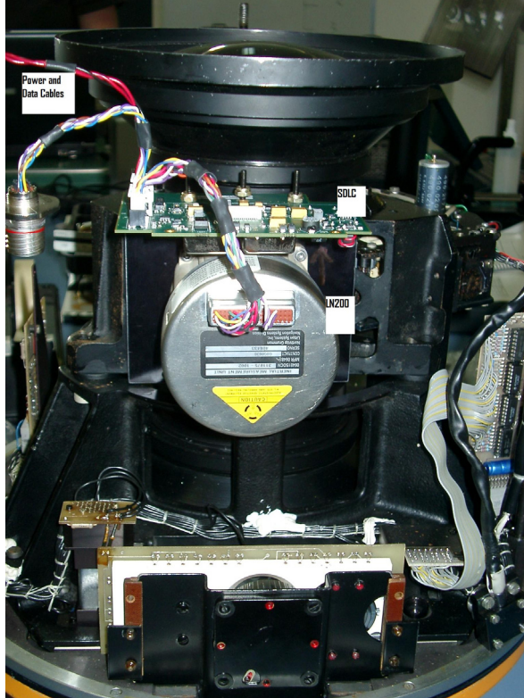
Figure 4. Board Level Integration of SPAN into LMK Camera
