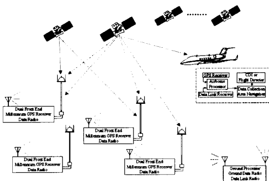
Figure 1. LTP System Block Diagram
