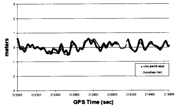
Figure 9. Minneapolis B-Value Data
