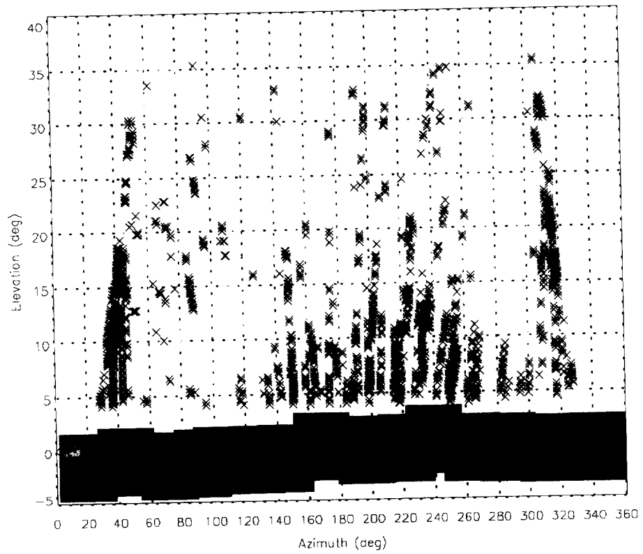
Figure 6. Minneapolis Site Ref 3 Multipath Plot
