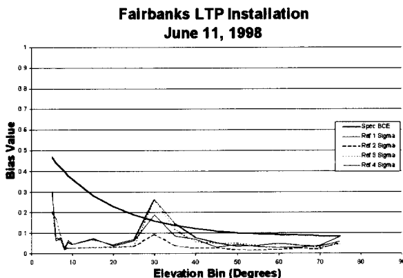
Figure 3. FAI Reference performance
