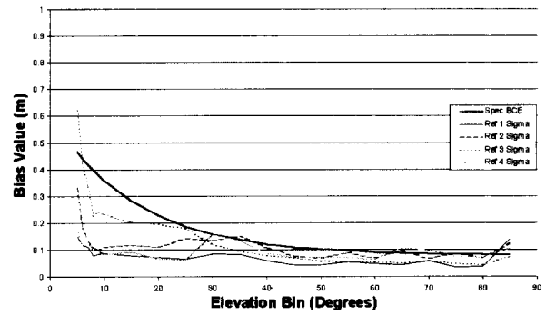
Figure 8. MSP Reference performance
