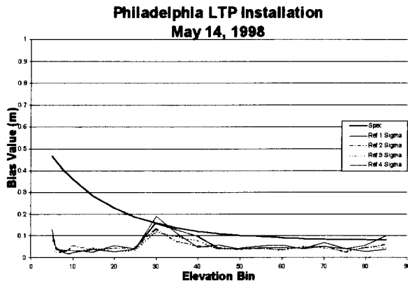
Figure 2. PHL Reference performance
