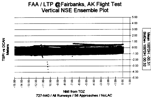
Figure 11. FAI Vertical NSE
