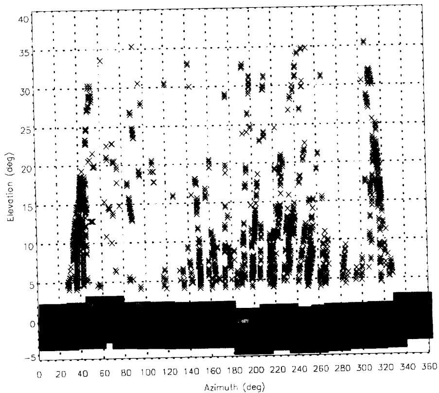
Figure 7. Site Ref 3 Multipath Plot - 180° Photo Shift
