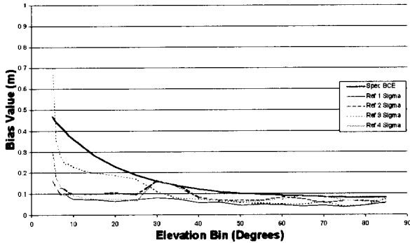
Figure 5. MSP Reference performance
