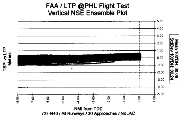
Figure 10. PHL Vertical NSE
