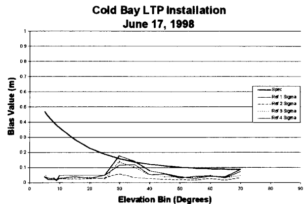
Figure 4. CDB Reference performance
