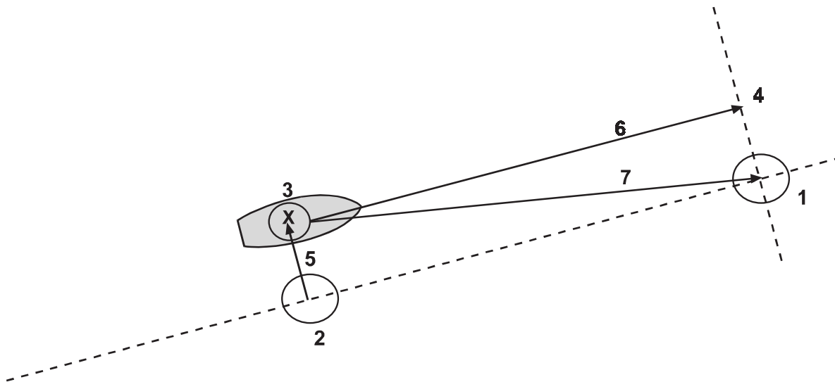
Figure C-5 Illustration of SETNAV Parameters
